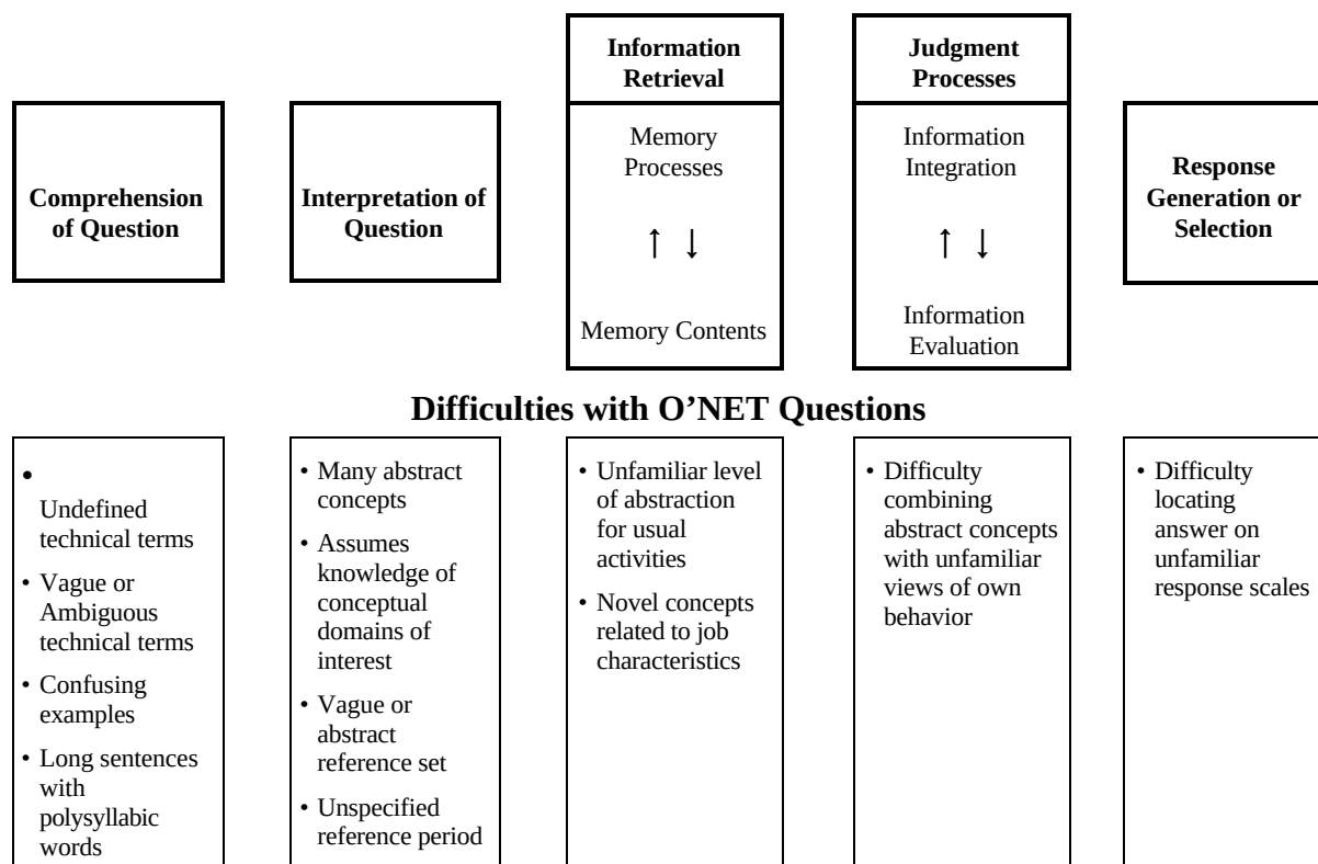
Figure 3. Problems with O*NET Questions Identified by Cognitive Process Model
