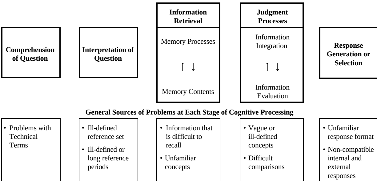
Figure 1. Cognitive Model of the Survey Response Process
